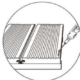
Last Piece of board could use 1 side grooved board, then, use screw to fix
