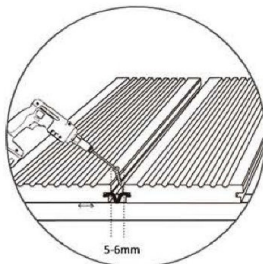
The decking board will have a gap about 5-6mm after installation
